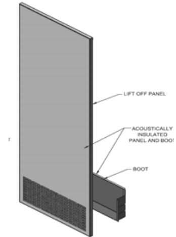
Two Piece Return Air Panel with boot and punched grille
