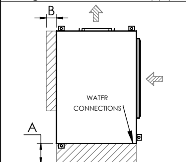
Arr. 4 Right Return, Back Supply
