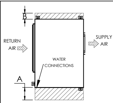
Arr. 1 Left Return, Right Supply
