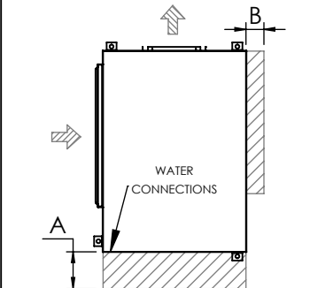
Arr. 3 Left Return, Back Supply
