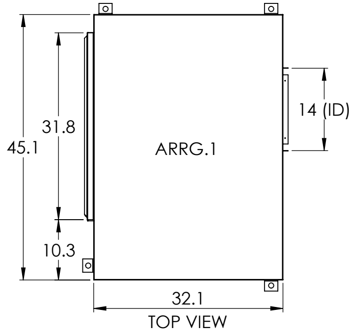
Arr. 1 Left Return, Right Supply
