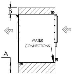
Arr. 2 Right Return, Left Supply
