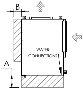
Arr. 4 Right Return, Back Supply
