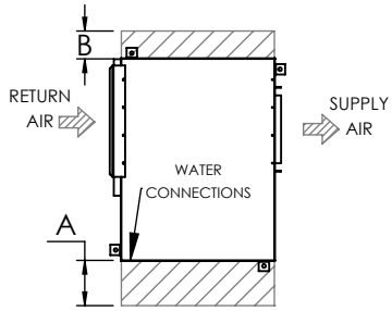
Arr. 1 Left Return, Right Supply
